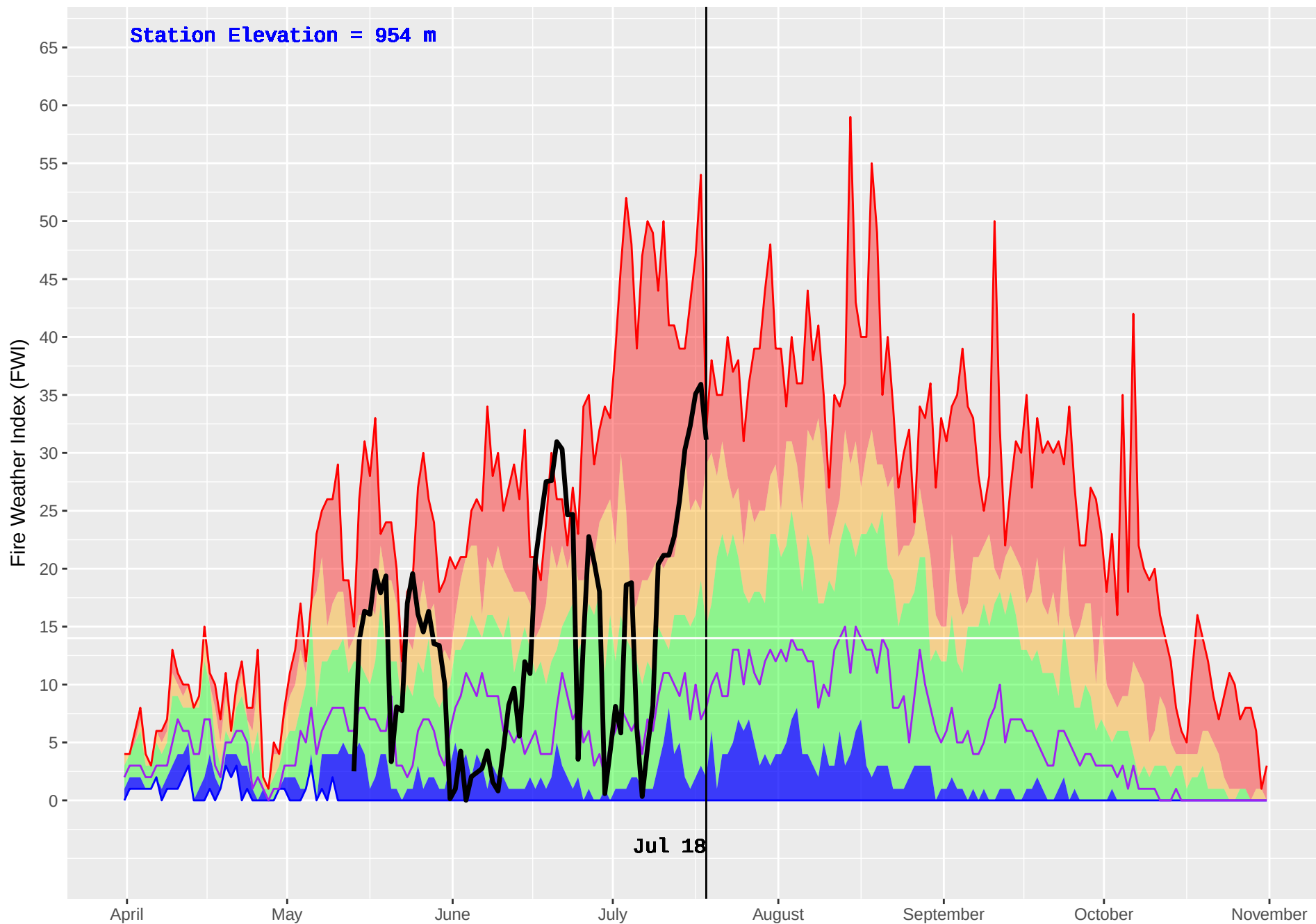
NADINA (179) : Historical (1985–2016) and Current (2018) Daily Fire Weather Index (FWI)
