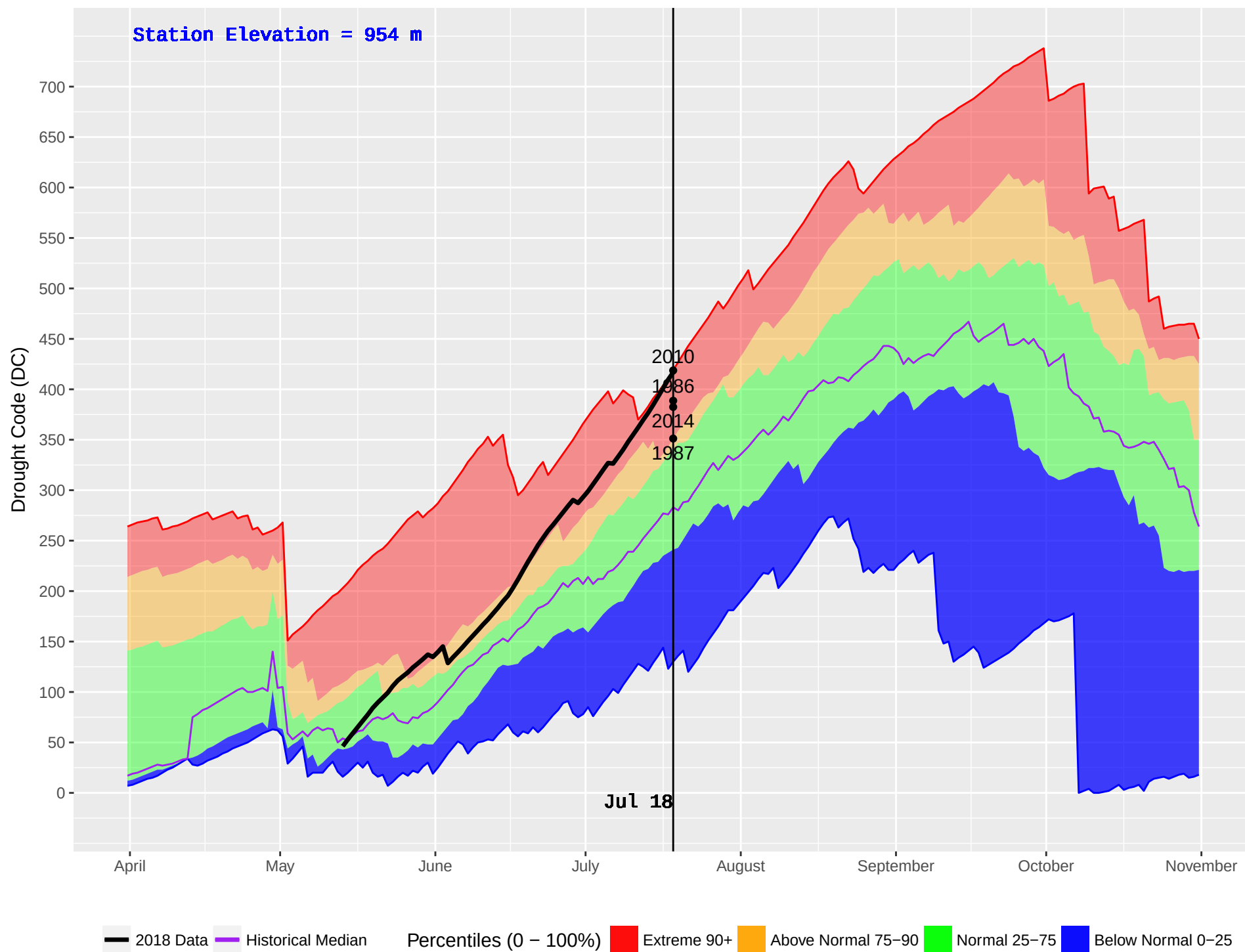
NADINA (179) : Historical (1985–2016) and Current (2018) Daily Drought Code (DC)
